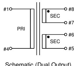
Schematic (Dual Output)
