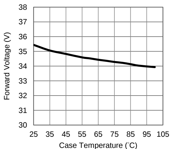
Fig 2. Case Temperature vs. Forward Voltage at 240mA.
