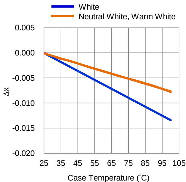
Fig 3. Case Temperature vs. Chromaticity Coordinate \Delta x at 240mA.
