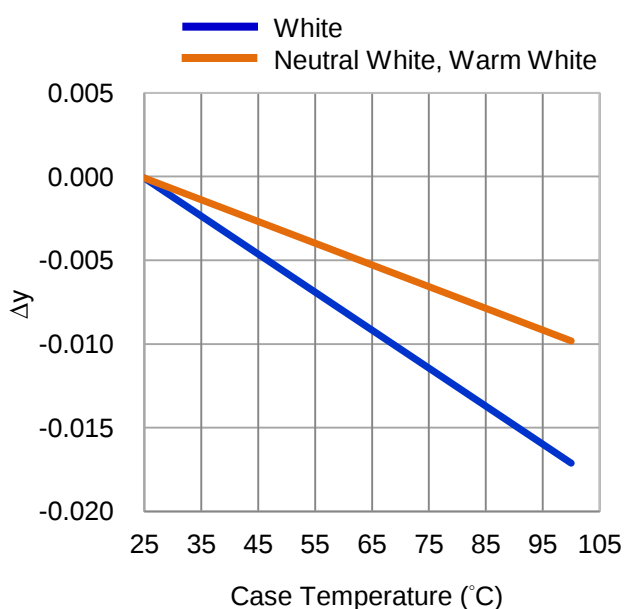
Fig 4. Case Temperature vs. Chromaticity Coordinate \Delta y at 240mA.
