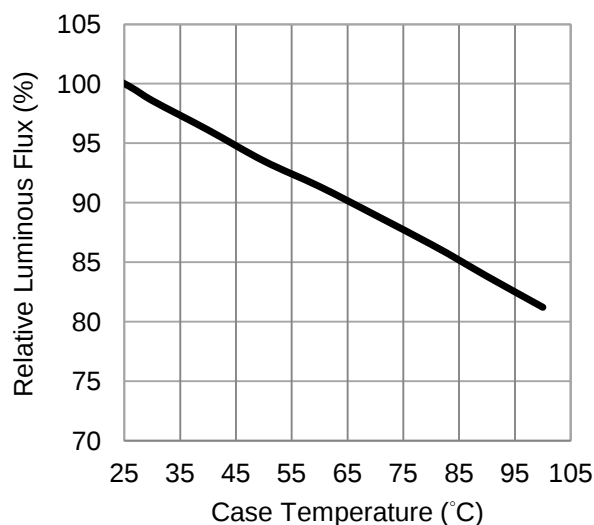
Fig 1. Case Temperature vs. Relative Luminous Flux at 240mA.
