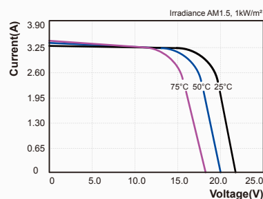
I-V Curves of PV module CL-SM60M at various cell temperatures
