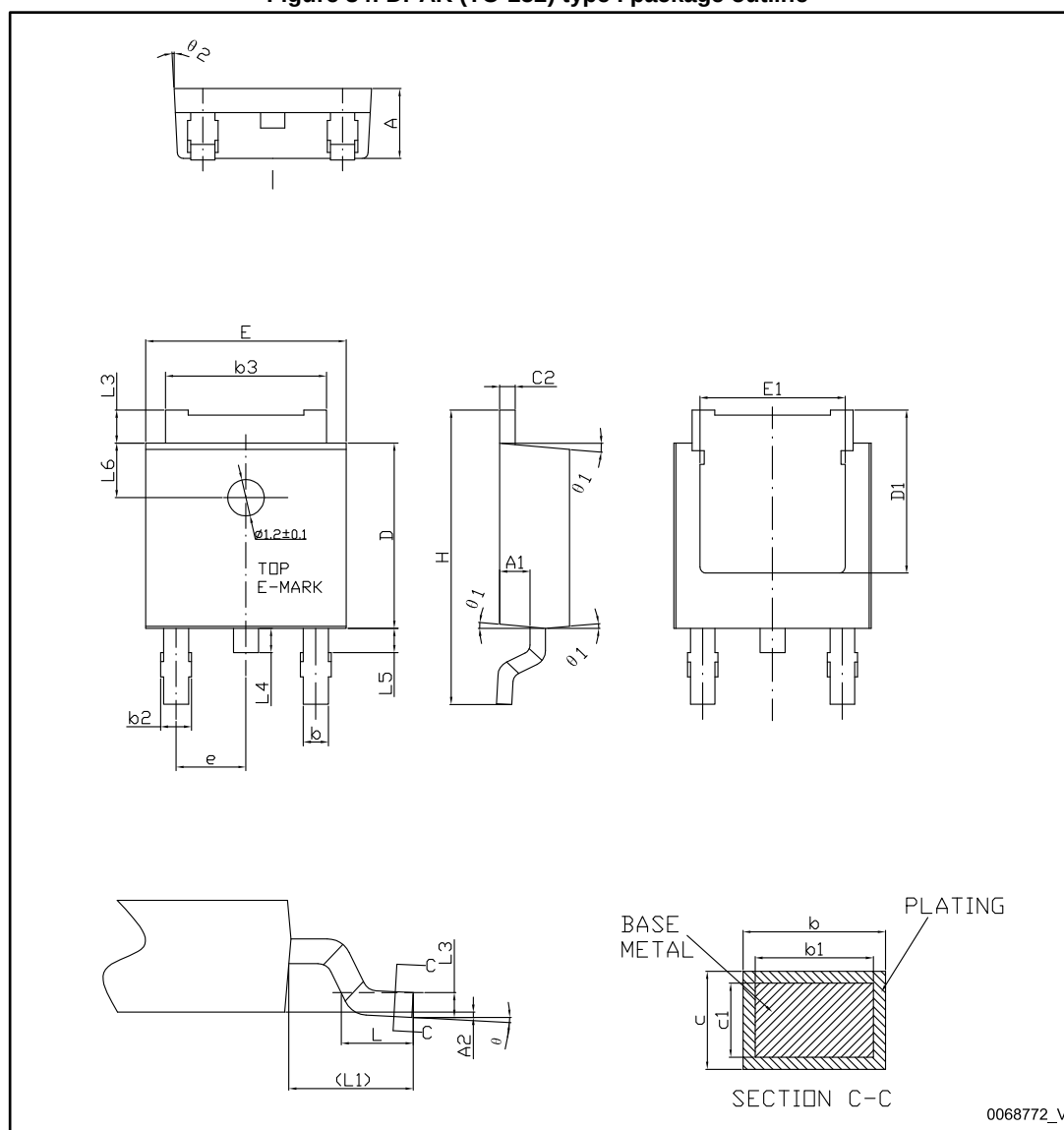
Figure 34: DPAK (TO-252) type I package outline
