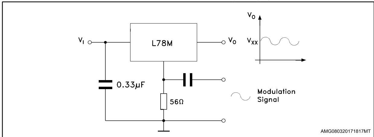
Figure 27: Power AM modulator (unity voltage gain, I_O \leq 0.5 )
