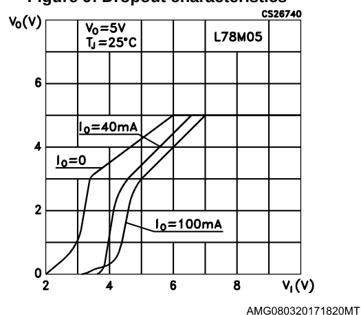
Figure 9: Dropout characteristics
