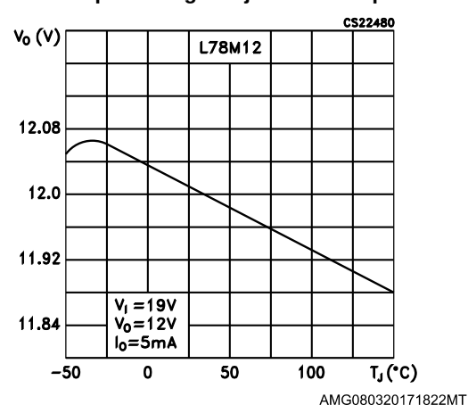
Figure 11: Output voltage vs junction temperature
