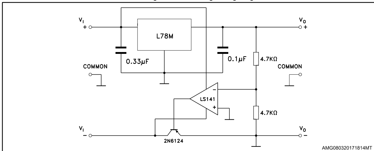
Figure 25: High input voltage circuit
