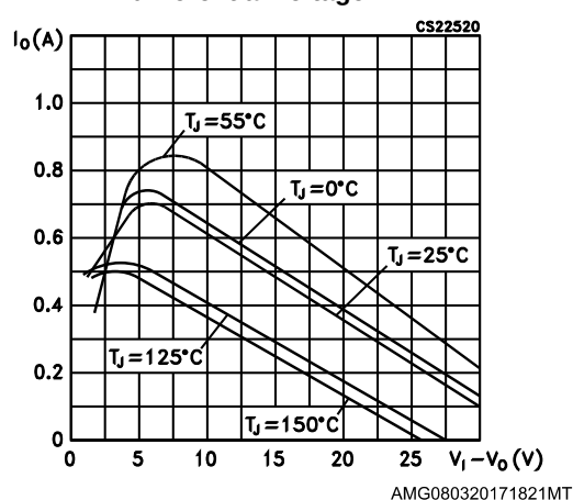
Figure 10: Peak output current vs input-output differential voltage
