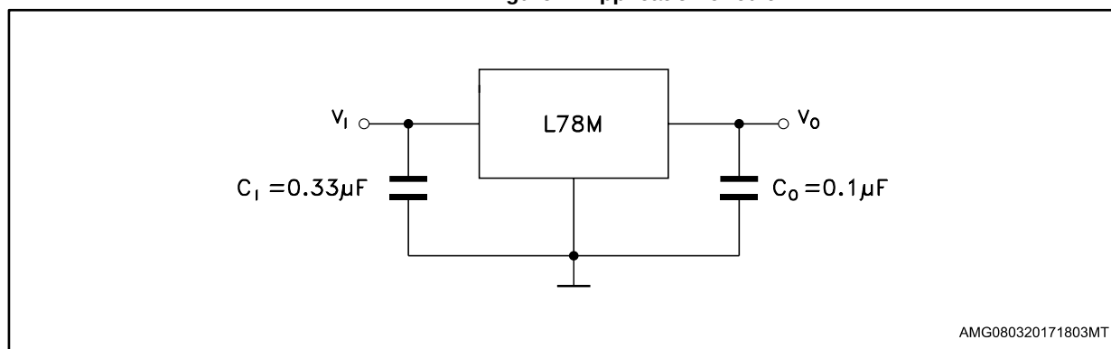
Figure 4: Application circuit
