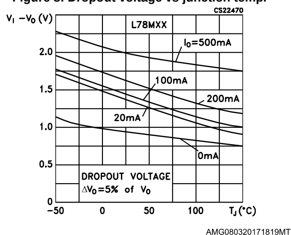
Figure 8: Dropout voltage vs junction temp.
