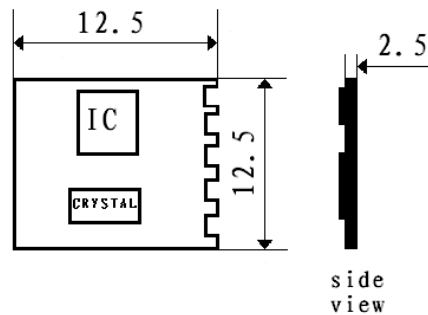
Figure2 CY89 Dimension
