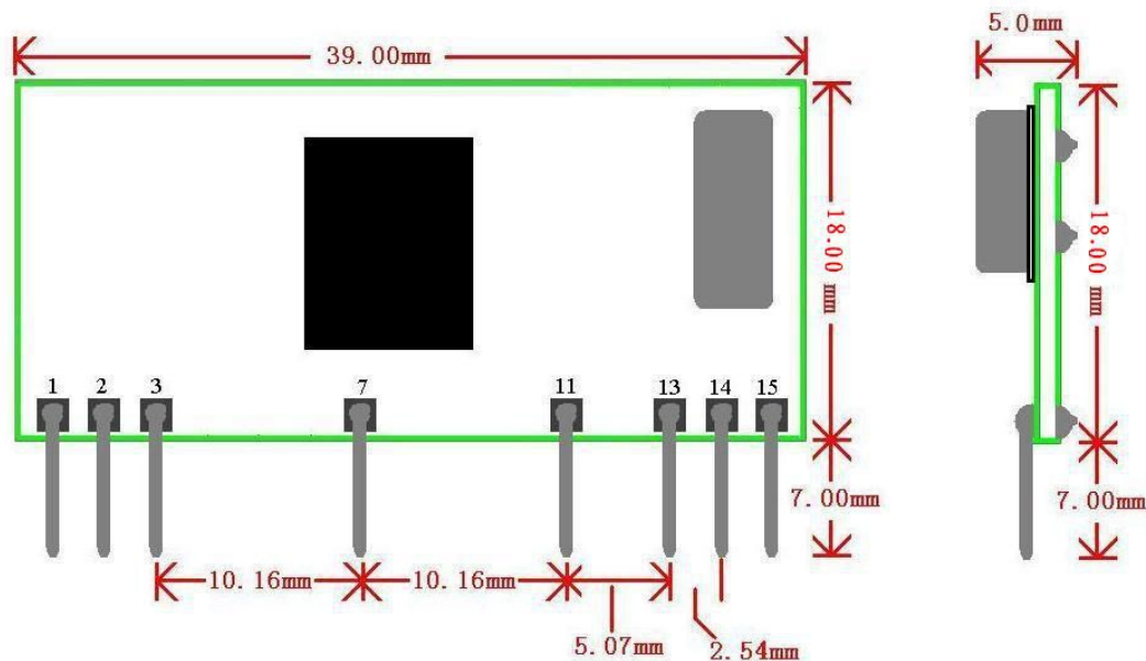
Figure2 CY78 Dimension
