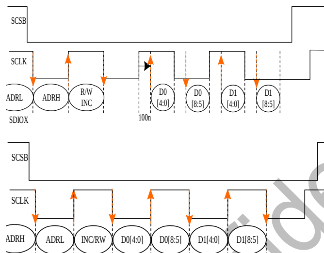
Figure 14 Parallel Port Read (Upper)/Write (Below) with Dual edge data latch
