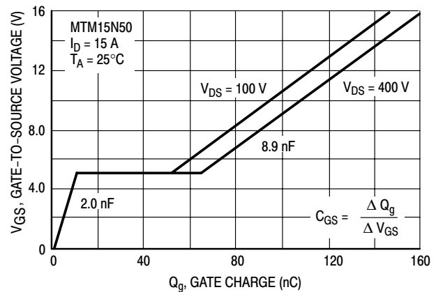
Figure 18. Gate-To-Source Voltage versus Gate Charge
