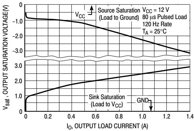
Figure 10. Drive Output Saturation Voltage versus Load Current
