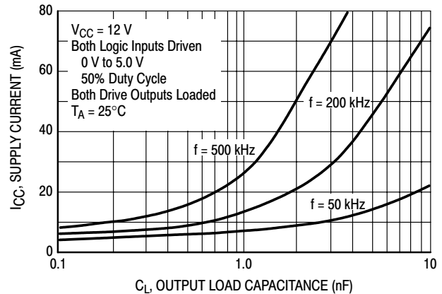
Figure 15. Supply Current versus Drive Output Load Capacitance
