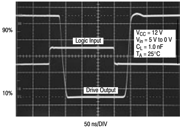
Figure 8. Propagation Delay
