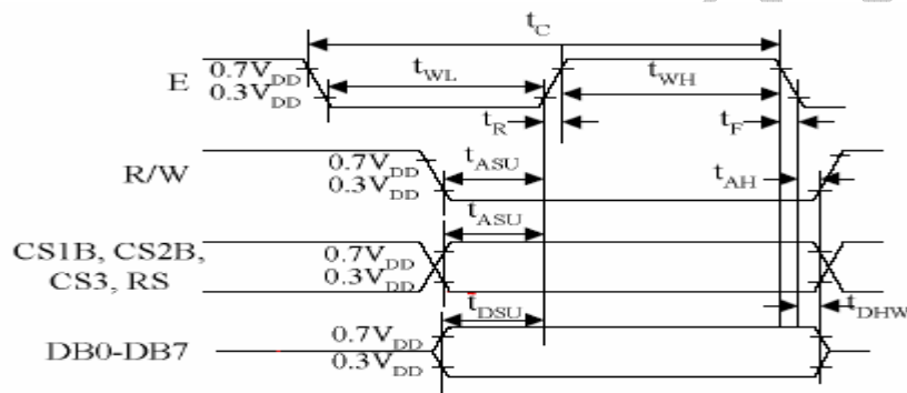
MPU Write Timing
