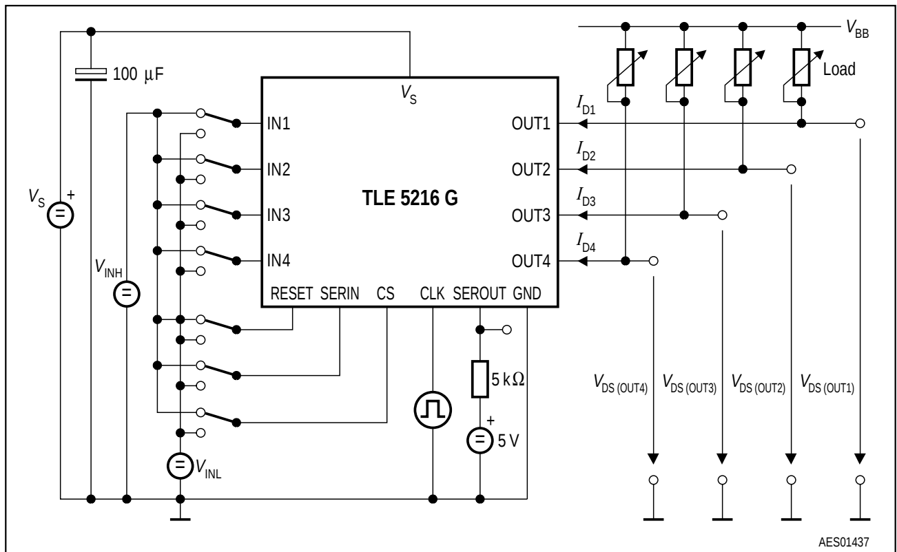
Figure 3 Test Circuit 1
