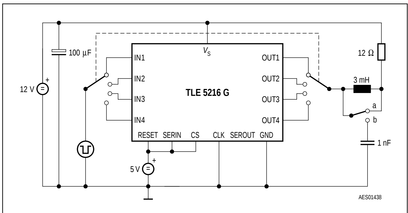
Figure 4 Test Circuit 2
