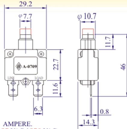
DIMENSION IN mm
