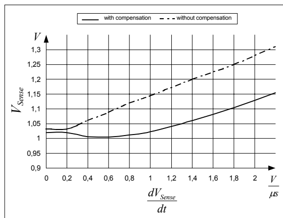
Figure 20 Overcurrent Shutdown
