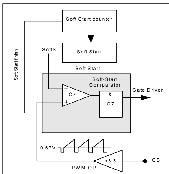
Figure 9 Soft Start
