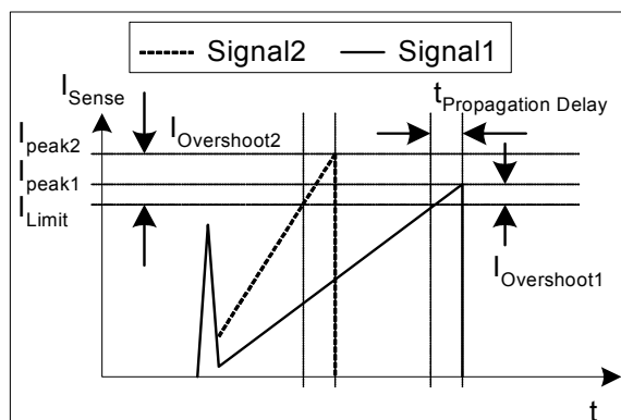
Figure 19 Current Limiting
