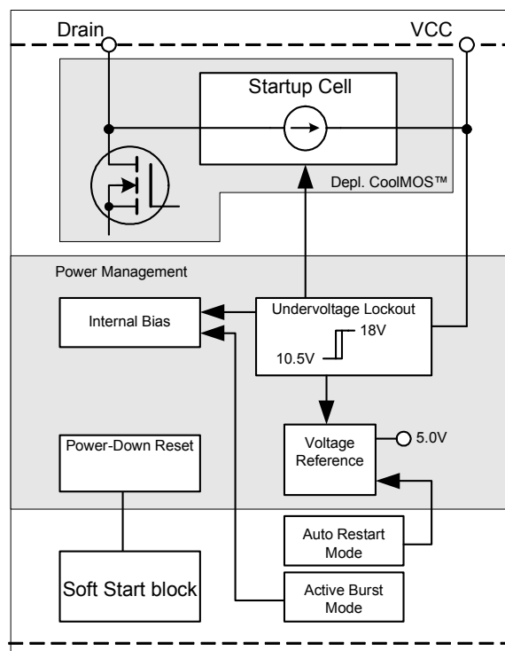
Figure 3 Power Management
