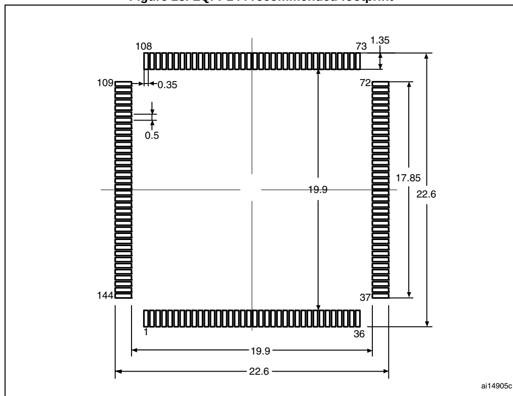
Figure 23. LQFP144 recommended footprint
