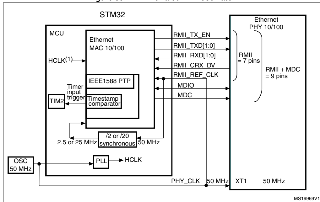
Figure 35. RMII with a 50 MHz oscillator
