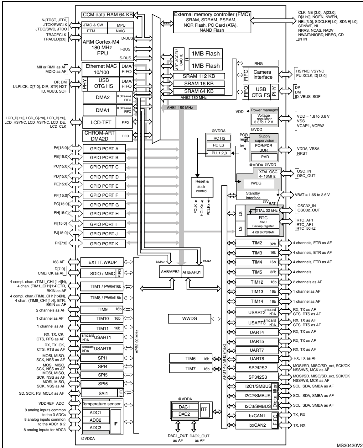
Figure 4. STM32F429xx block diagram
