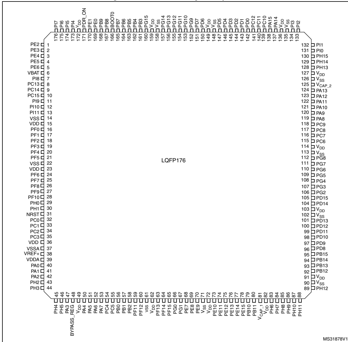
Figure 14. STM32F42x LQFP176 pinout
