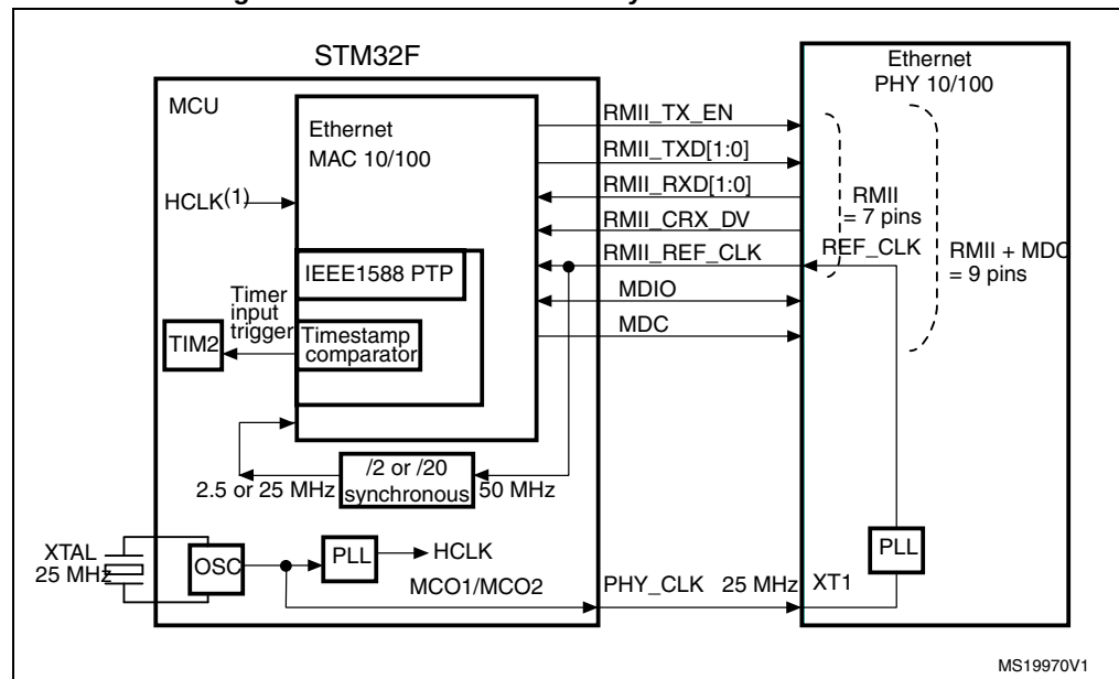
Figure 36. RMII with a 25 MHz crystal and PHY with PLL
