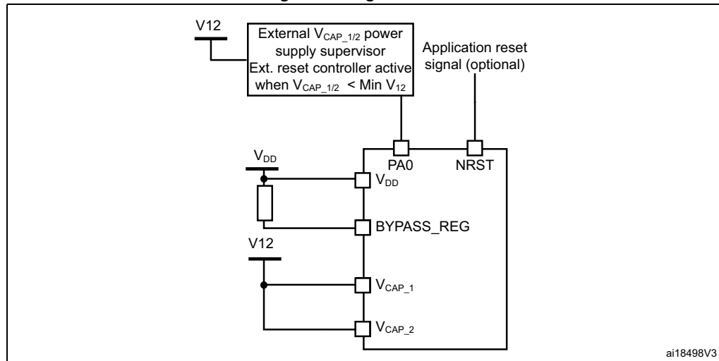
Figure 8. Regulator OFF
