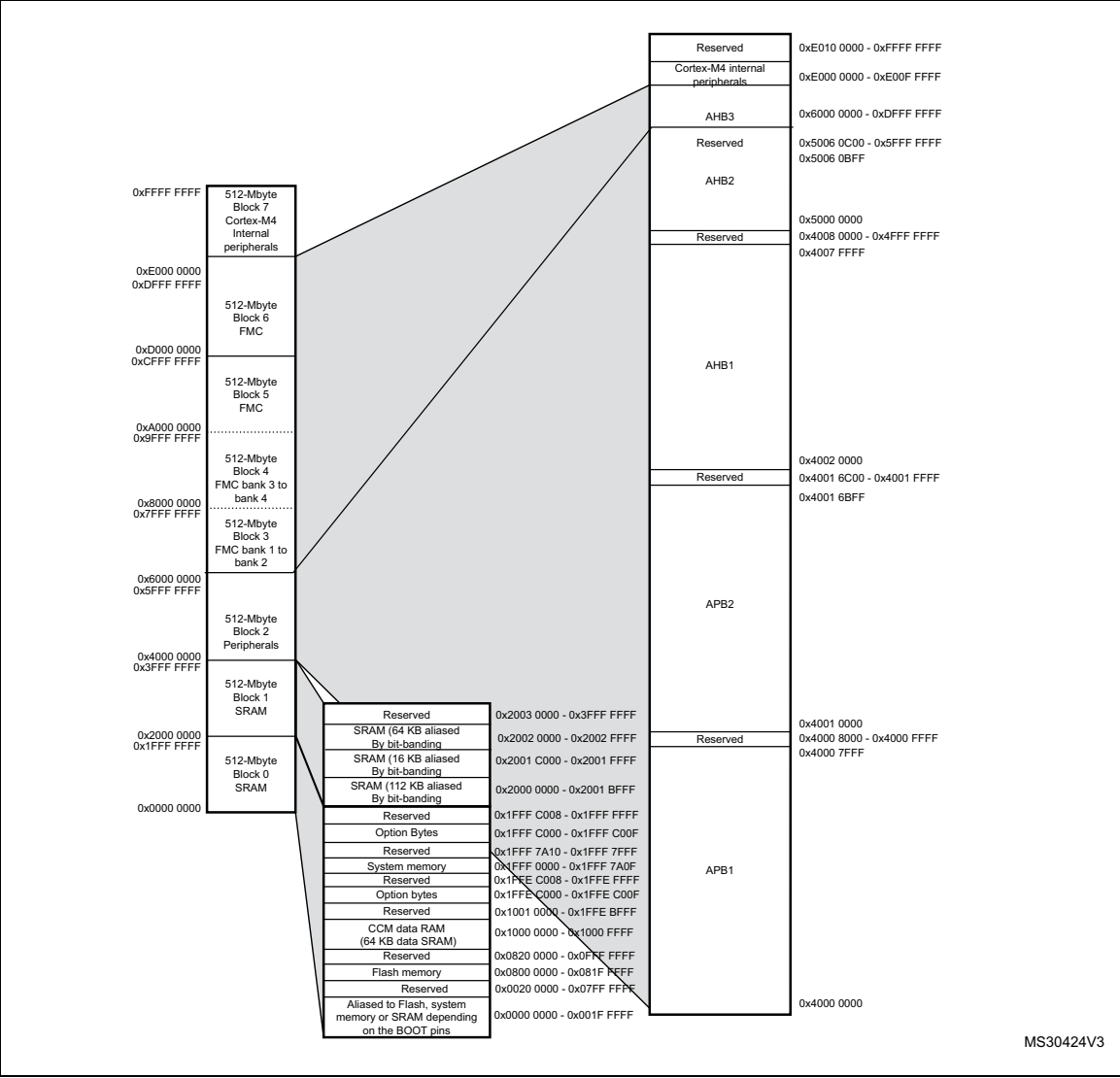
Figure 18. Memory map
