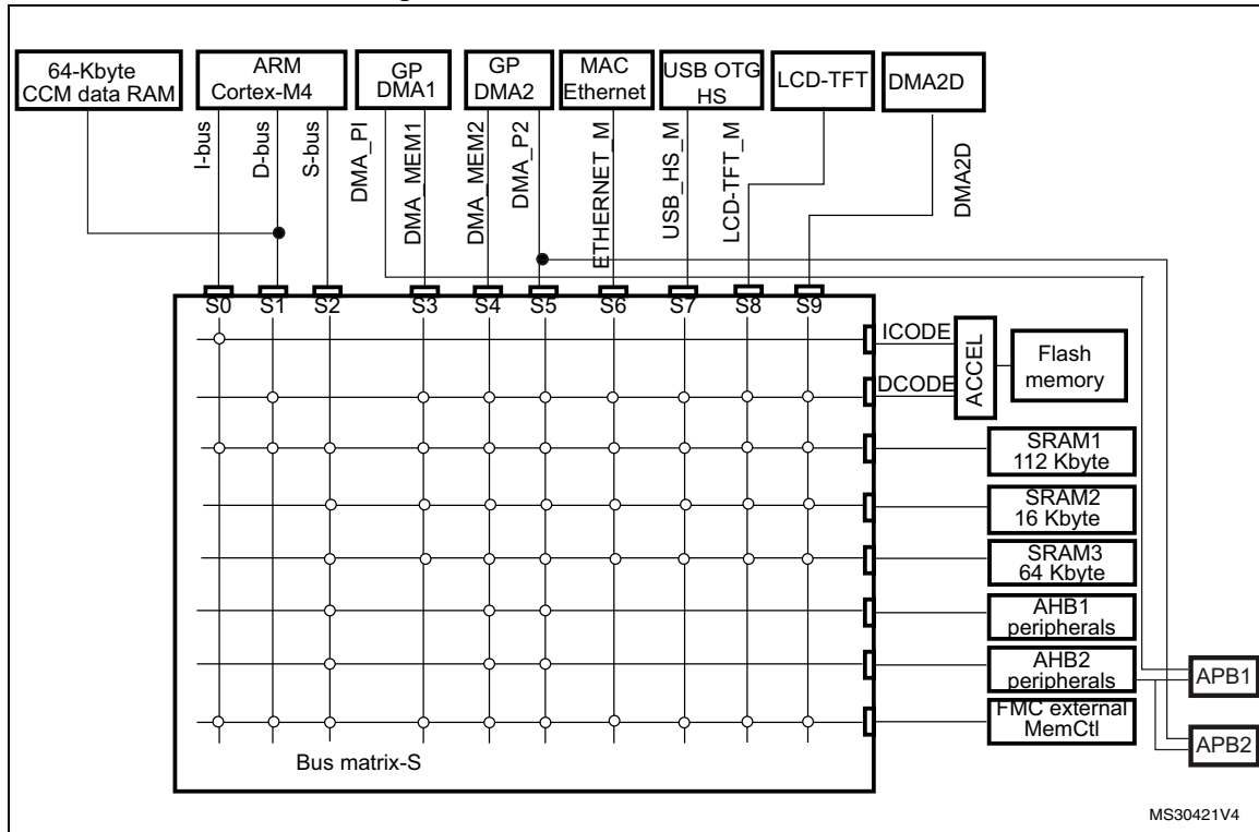
Figure 5. STM32F429xx Multi-AHB matrix
