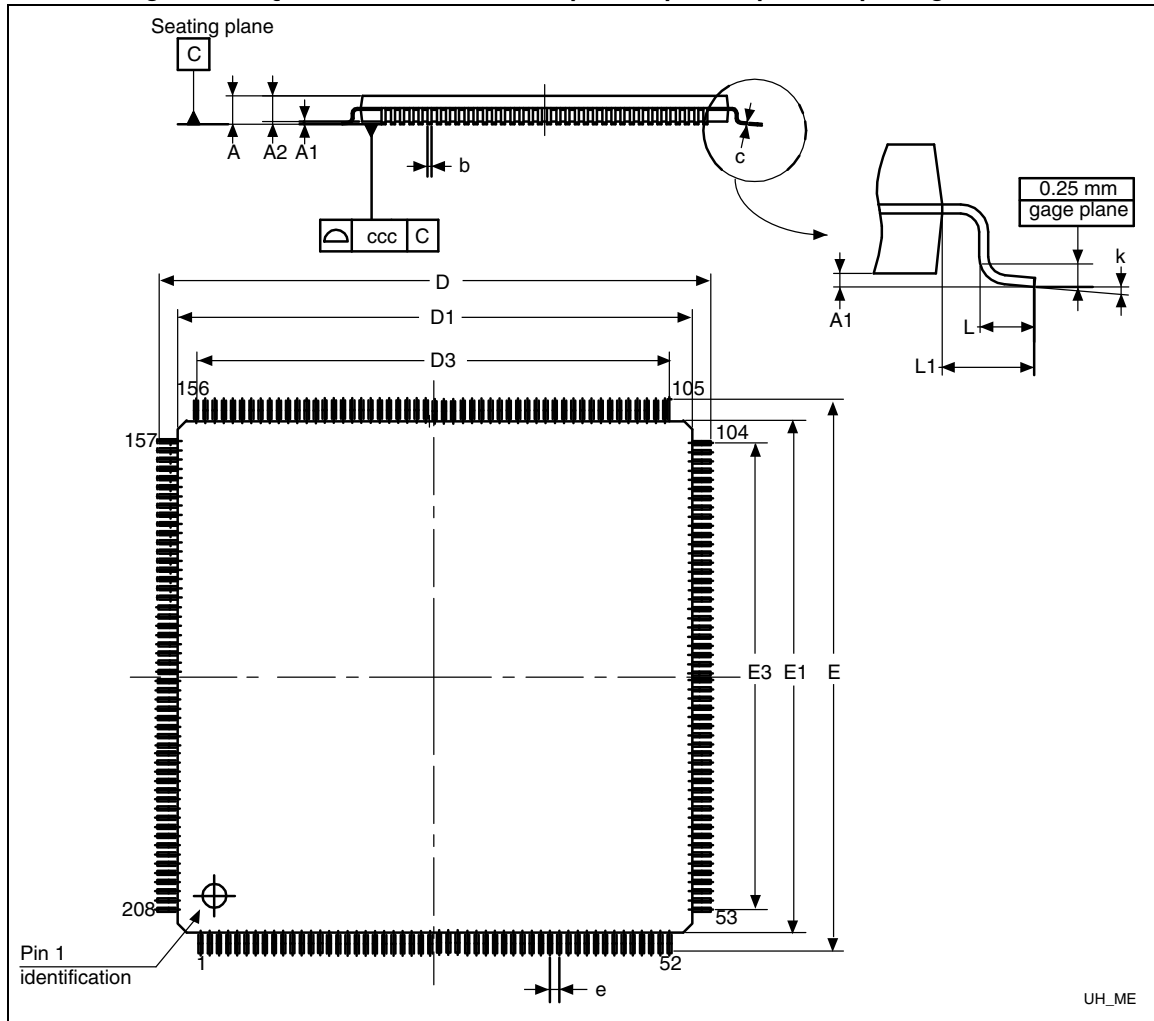
Figure 26. LQFP208, 28 x 28 mm, 208-pin low-profile quad flat package outline
