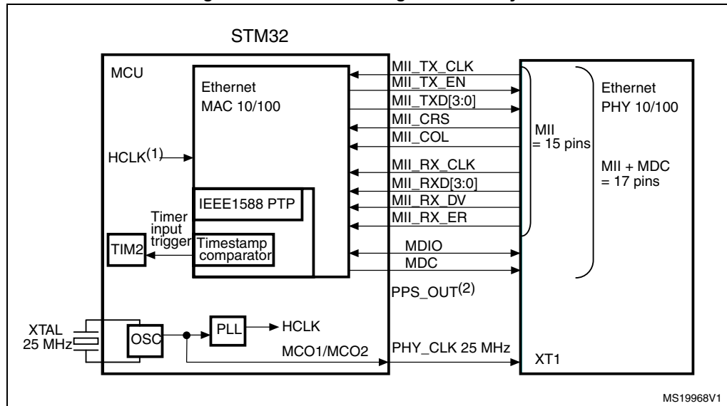
Figure 34. MII mode using a 25 MHz crystal
