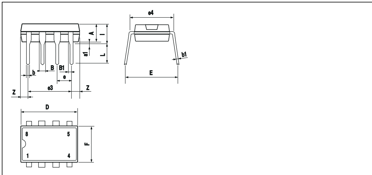
Figure 3. 8-Pin Package
