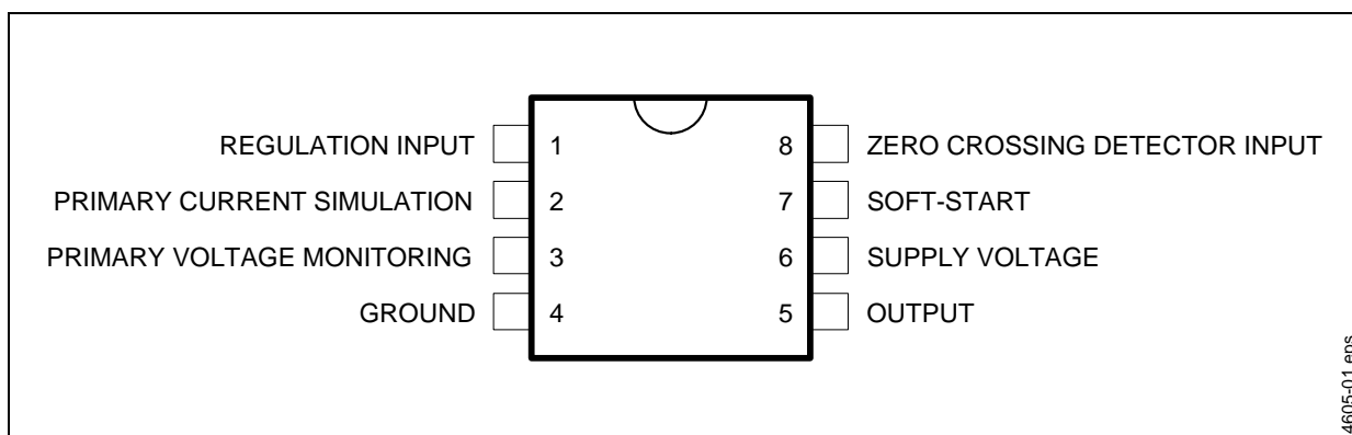
Figure 1. Pin Connections
