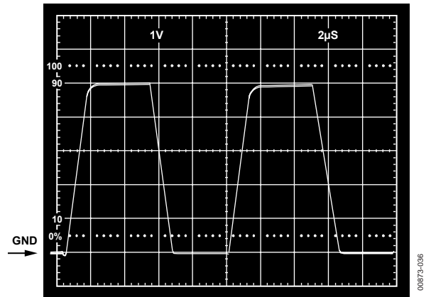
Figure 36. V_S = 5\text{ V}, 0\text{ V} ; Gain of Two Inverter Response to 2.5 V Step, Centered -1.25\text{ V} Below Ground
