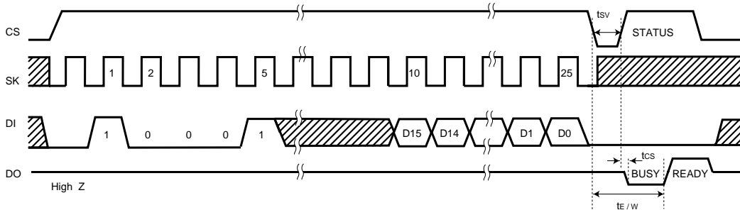
Fig. 5 Write all address cycle timing. (WRAL)
