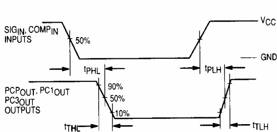
Figure 1. Switching Waveforms
