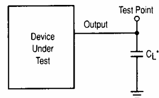
Figure 6. Test Circuit
