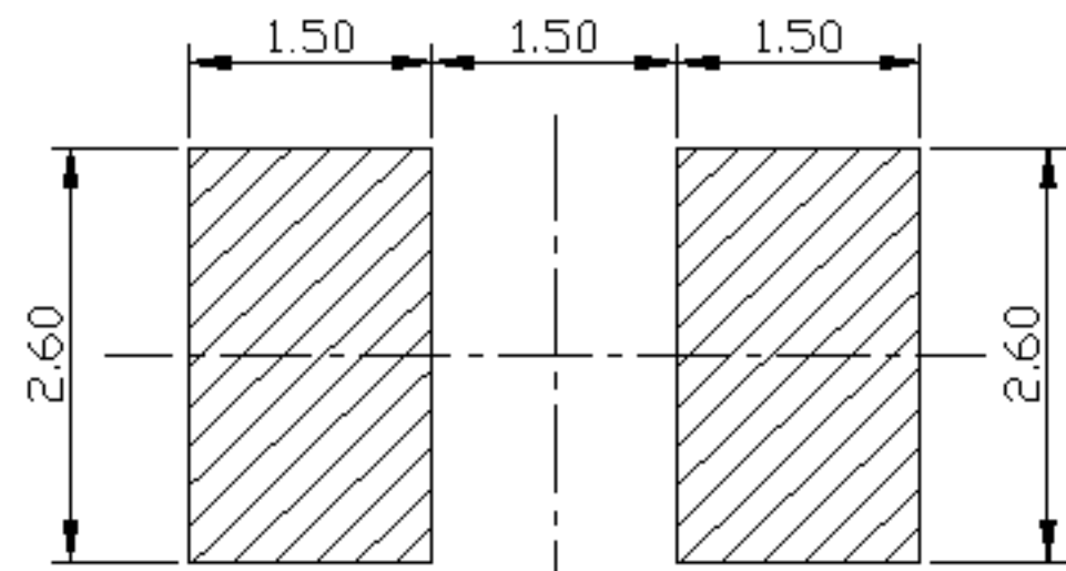
Recommended Soldering Pad
