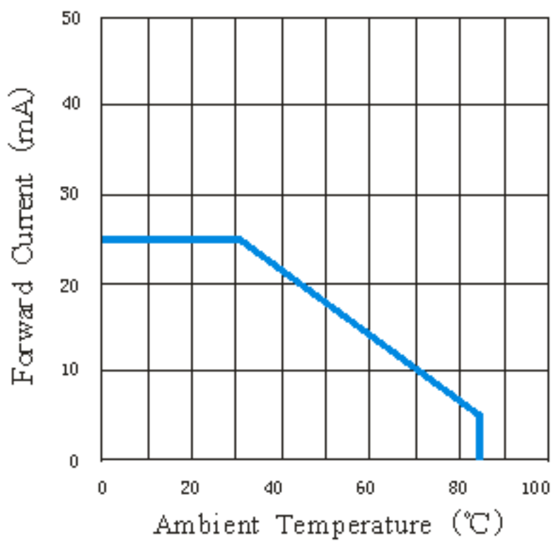
Forward Current Derating Curve
