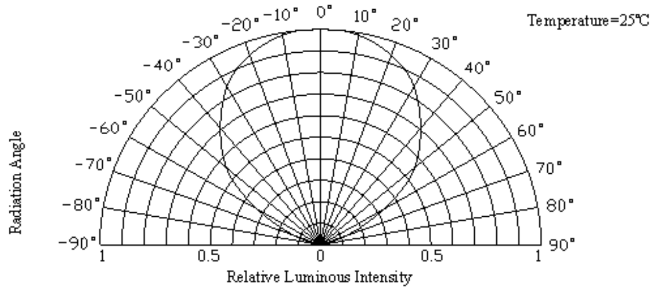
Radiation Diagram
