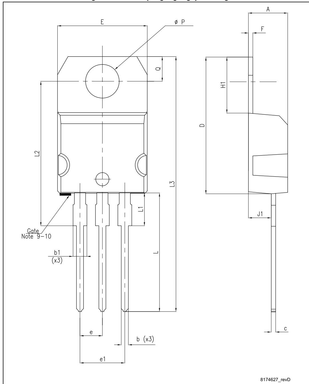
Figure 8. TO-220 (single gauge) drawing
